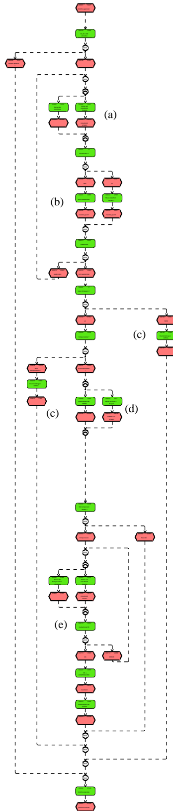
Figure 3: Structure of the agent’s meta workflow in EPC notation
